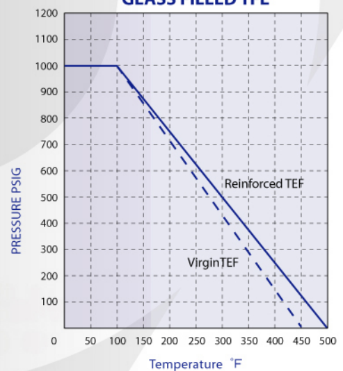
R-TFE SEATS GLASS FILLED TFE
